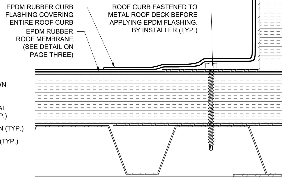
PH1 CURB INSTALLATION 6" = 1'-0"
