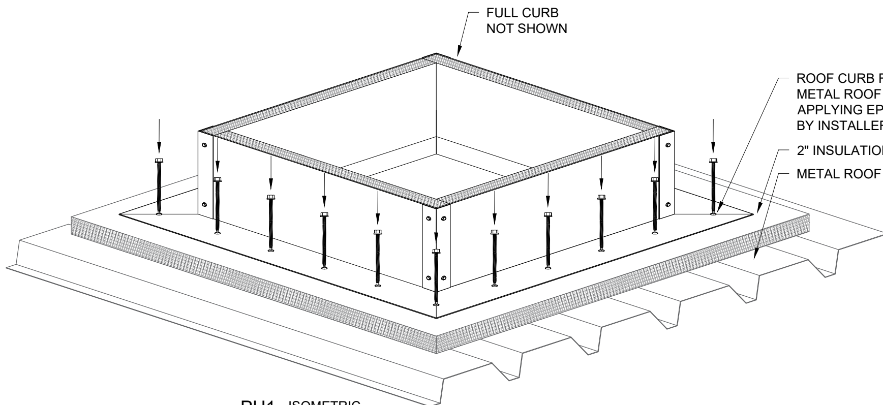
PH1 ISOMETRIC 1-1/2" = 1'-0"
